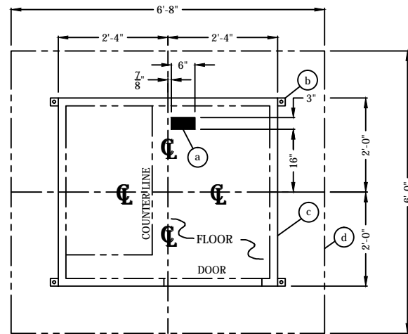
SERVICE ENTRANCE/ANCHOR BOLT LAYOUT
