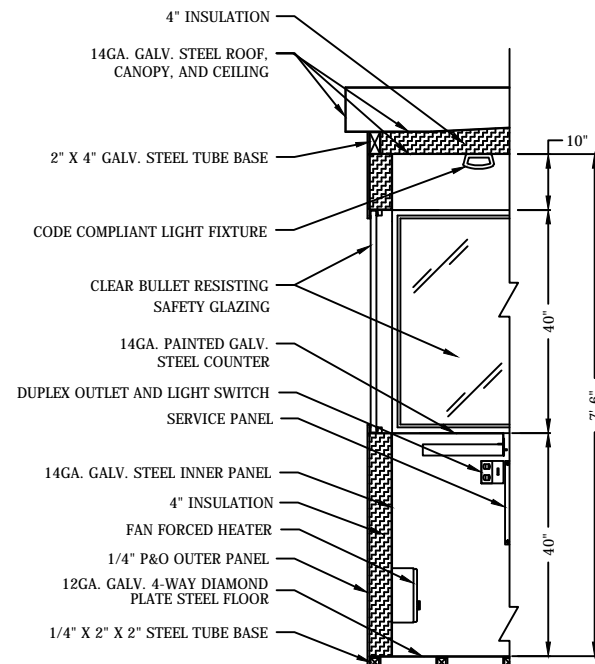
S1 SECTION NO SCALE
